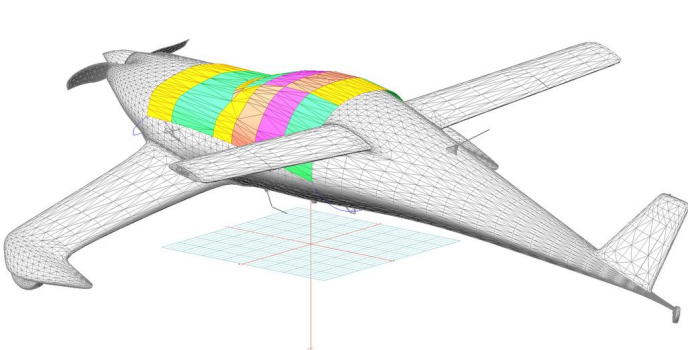
Rutan Quickie Canopy Cover, 3D model
