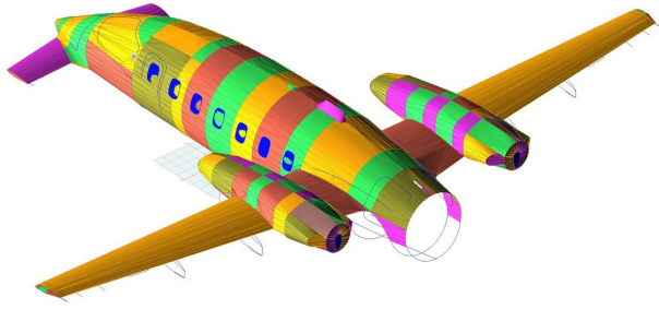
Piaggio P180 Fuselage, Canard, Wing & Engine Covers, 3D model
