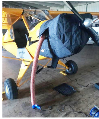
Legend Cub AL3 Insulated Engine Cover with special preheater access vent and attachment detail and fully enclosed under cowling.
