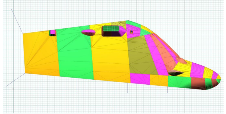
Agusta Leonardo A169 Bubble Cover with Wire Strike, 3D model
